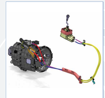
Cable type shift mechanism
